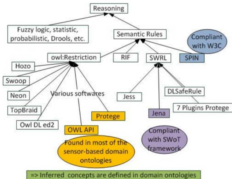
Figure 1 Interoperability issues regarding reasoning
